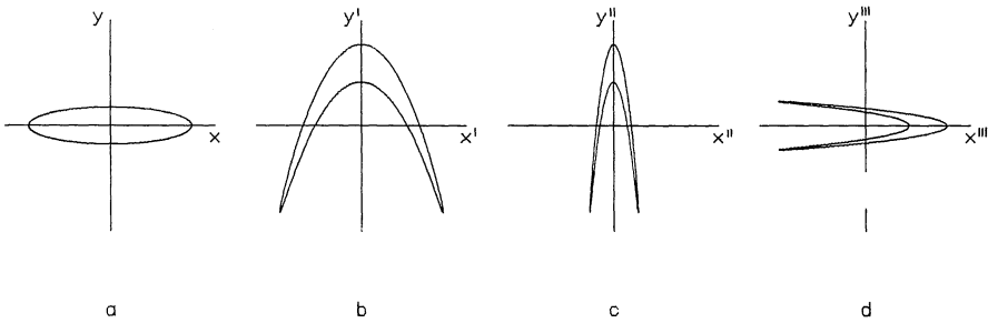
Fig. 1. The initial area a is mapped by T' into b , then by T'' into c , and finally by T''' into d
