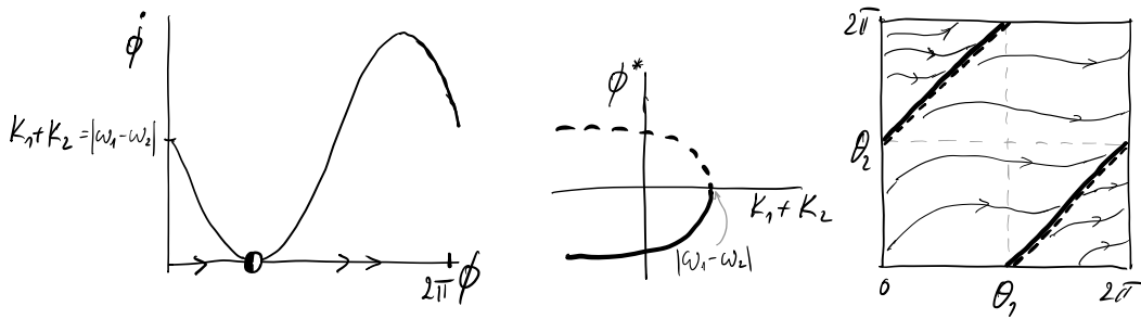
Figure 8: (Left) One-dimensional phase portrait of phase difference \phi given by (9) featuring a half-stable fixed point. (Middle) Bifurcation diagram where bifurcation point (K_1 + K_2)^* = |\omega_1 - \omega_2| . (Right) 2\pi -periodic square showing a half-stable (bold line) non-isolated fixed point or a trajectory on the torus corresponding to the fixed point shown on the left.
