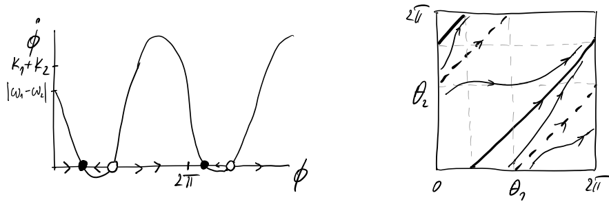
Figure 7: (Left) One-dimensional phase portrait of phase difference \phi given by (9) where all trajectories are approaching the stable fixed point. (Right) 2\pi -periodic square showing stable (solid bold line) and unstable (dashed bold line) non-isolated fixed points or trajectories on a torus corresponding to fixed points defined by (10) and shown on the 1-D phase portrait on the left. The slope of stable and unstable phase-locked solutions is 1, since \omega^* = \dot{\theta}_1 = \dot{\theta}_2 .
