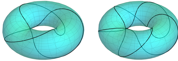
Figure: Two examples of closed trajectories defined by Sys. (1) as they appear on the surfaces of tori. (Left) Trefoil knot ( p = 3 , q = 2 ). (Right) Cinquefoil knot ( p = 5 , q = 2 ).
