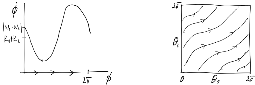
Figure 9: (Left) One-dimensional phase portrait of phase difference \phi given by (9). (Right) Flow on the 2\pi -periodic square corresponding to the phase portrait shown on the left.
