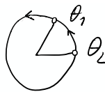
Figure 1: Circular stadium where the angular positions of two runners are shown with \theta_1(t) and \theta_2(t) .
