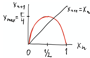
Figure 6: The logistic map shown with the red curve and the diagonal where x_{n+1} = x_n .
