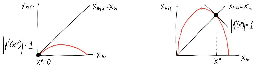
Figure 8: (Left) Map slope at the fixed points x^* = 1 - 1/r (same as the trivial cases x^* = 0 = 1 ) for r = 1 . (Right) Map slope at the fixed points x^* = 1 - 1/r for r = 3 .
