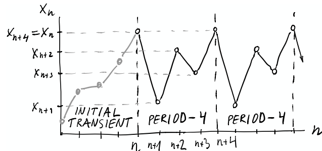
Figure 12: Period-4 orbit with its repeated iterates as they appear in the logistic map.
