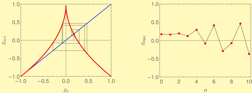
Figure 2: (Left) Cobweb diagram of the normalised Lorenz map showing the first ten iterates for z_0 \approx z^* where the fixed point z^* is unstable , since |f'(z^*)| > 1 . The Lorenz map has property |f'(z)| > 1, \forall z in the map basin. (Right) Lorenz map iterates corresponding to the cobweb diagram shown on the left.
