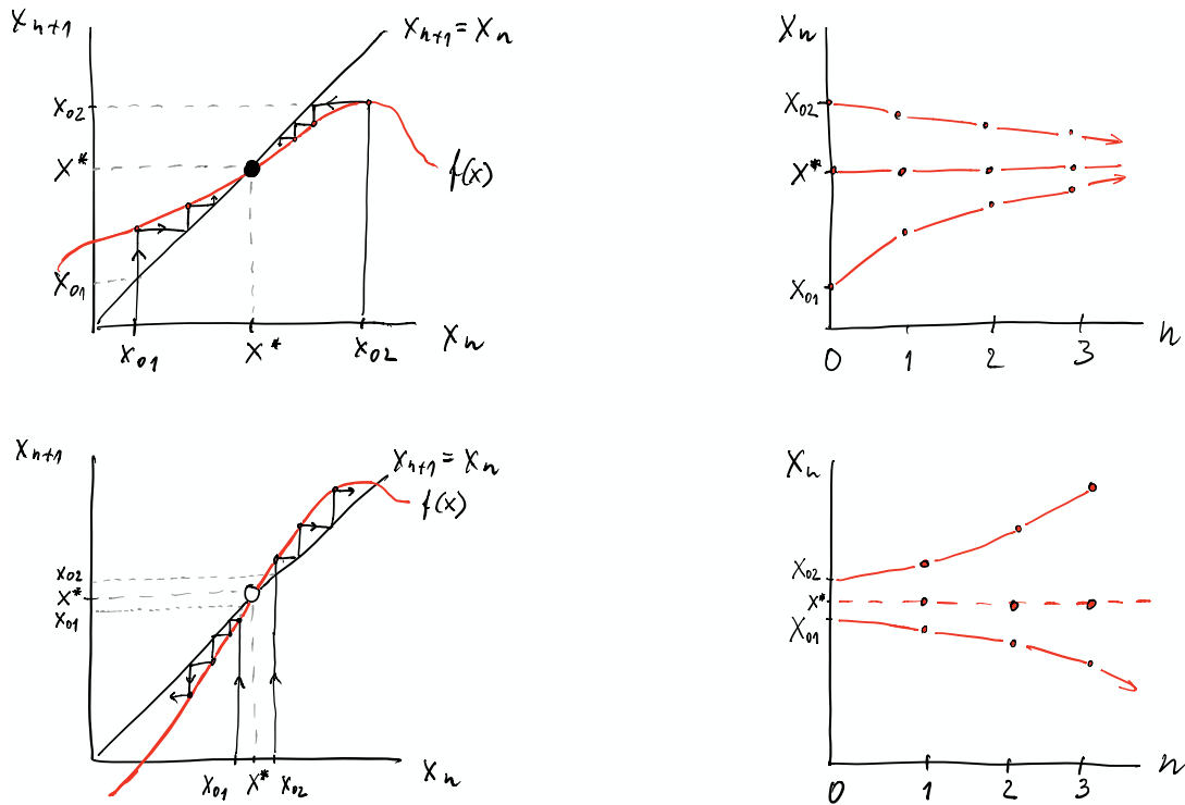
Figure 4: (Top-left) Stable fixed point x^* (a period-1 point) of a one-dimensional map given by x_{n+1} = f(x_n) where |f'(x^*)| < 1 is shown with the filled bullet. (Top-right) Three sets of map iterates x_n shown for initial conditions x_{01} , x^* and x_{02} corresponding to the cobweb diagram shown on the left. (Bottom-left) Unstable fixed point x^* (a period-1 point) shown with the empty bullet where |f'(x^*)| > 1 . (Bottom-right) Three sets of map iterates x_n shown for initial conditions x_{01} , x^* and x_{02} corresponding to the cobweb diagram shown on the left.
