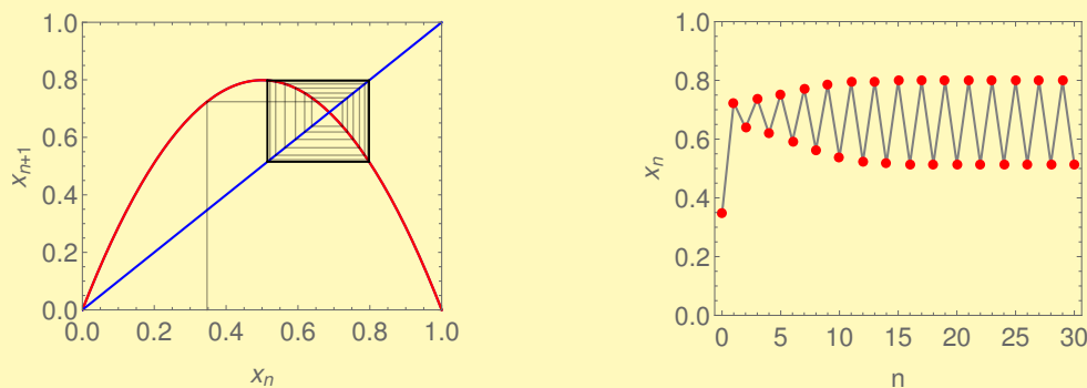
Figure 10: (Left) Cobweb diagram of the logistic map shown for r = 3.19 \geq 3 featuring the stable period-2 point. (Right) Map iterates corresponding to the cobweb diagram shown on the left.
