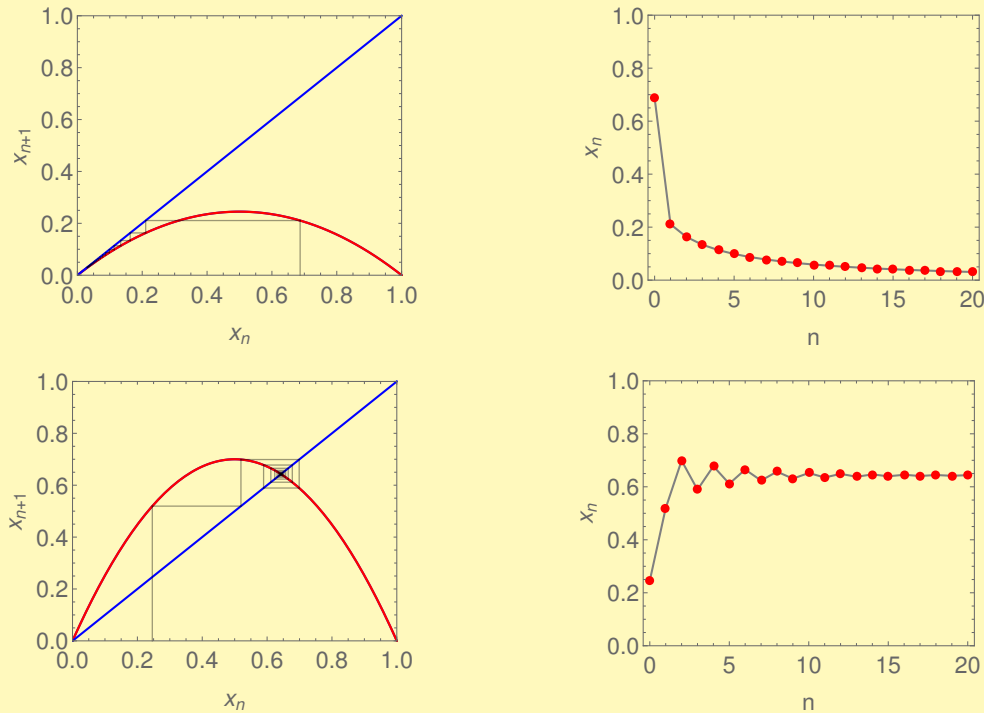
Figure 9: (Top-left) Cobweb diagram of the logistic map shown for r = 0.98 < 1 . The fixed point x^* = 0 . (Top-right) Map iterates corresponding to the cobweb diagram shown on the left. (Bottom-left) Cobweb diagram of the logistic map shown for interval 1 < r < 3 with r = 2.82 . The fixed point x^* = 1 - 1/r . (Bottom-right) Map iterates corresponding to the cobweb diagram shown on the left.
