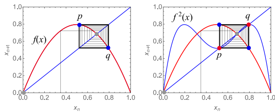
Figure: The logistic map where r = 3.18 and x_0 = 0.35 . Fixed points (f.p.s) in the case where r < 3 are shown with the grey bullets. Period-2 points of f(x) map for r \geq 3 are shown with the blue bullets. The fixed points of f^2(x) map for r \geq 3 are shown with the red bullets.
