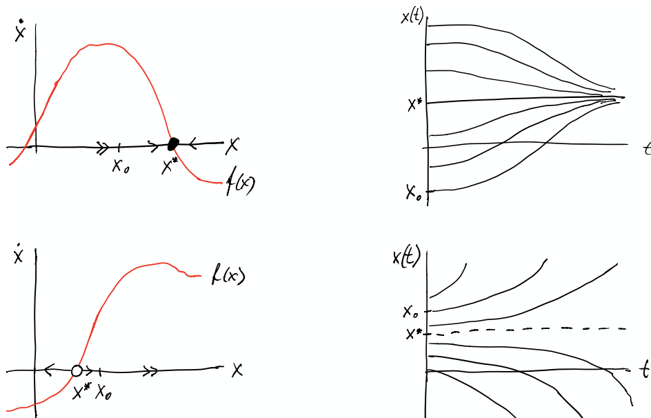
Figure 3: (Top-left) Stable fixed point x^* of a one-dimensional system given by \dot{x} = f(x) where f'(x^*) < 0 is shown with the filled bullet. (Top-right) A family of time-series solutions shown for several initial conditions positioned close to x^* . The solutions correspond to the phase portrait shown on the left. (Bottom-left) Unstable fixed point x^* shown with the empty bullet where f'(x^*) > 0 . (Bottom-right) A family of time-series solutions shown for several initial conditions positioned close to x^* . The solutions correspond to the phase portrait shown on the left.
