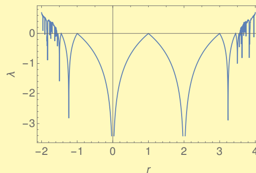
Figure 7: The Lyapunov exponent of the logistic map as a function of the growth rate r . Calculation uses 5000 iterations for every r value plotted.
