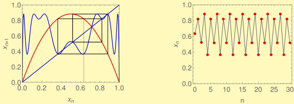
Figure 11: (Left) Cobweb diagram of the logistic map shown for r = 3.535 \geq 1 + \sqrt{6} featuring the stable period-4 point. The blue graph shows fourth iterate map f^4 . (Right) Map iterates corresponding to the cobweb diagram of map f shown on the left.
