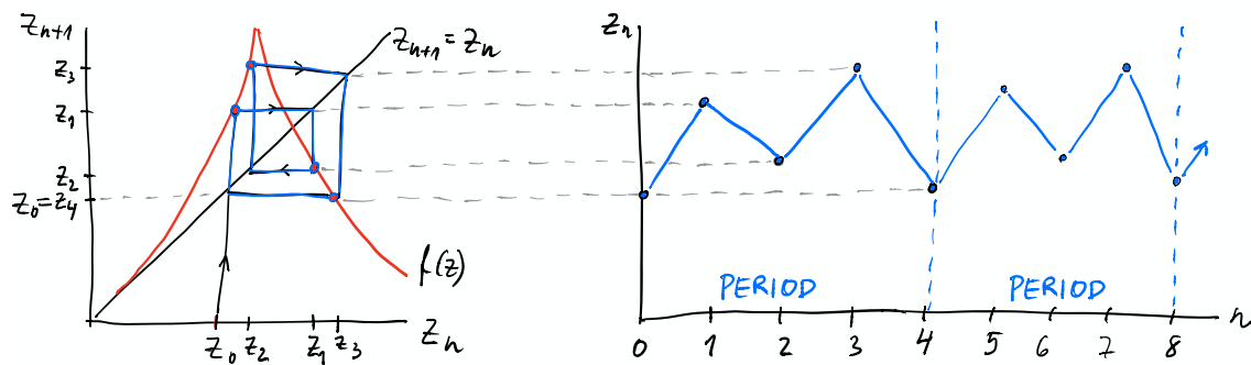
Figure 5: (Left) Period-4 orbit, shown with the blue graph, where z_{n+4} = z_n . (Right) The Lorenz map iterates z_n corresponding to the cobweb diagram shown on the left. The map iterates are repeat every four iterates.
