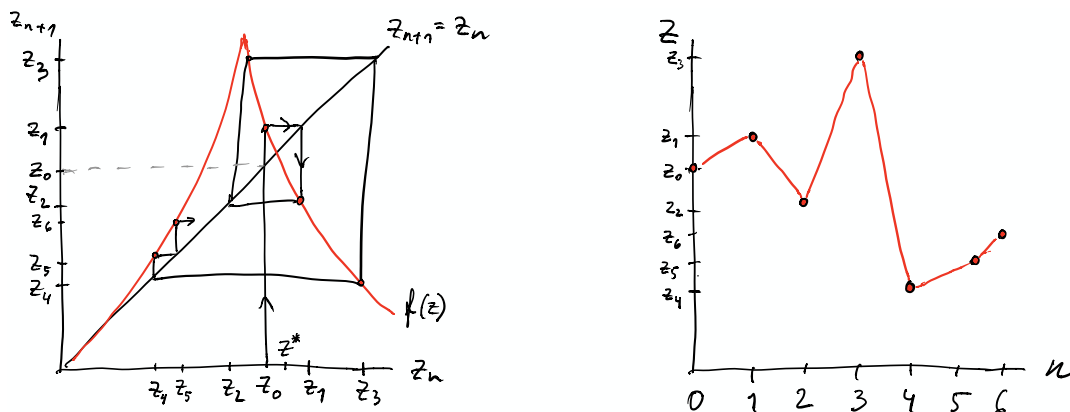
Figure 1: (Left) Cobweb diagram of the Lorenz map. (Right) The Lorenz map iterates corresponding to the cobweb diagram shown on the left.
