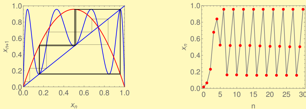
Figure 13: (Left) Period-3 orbit of the logistic map can be found in the period-3 window of the orbit diagram, see Slide 11. Here, showing the trajectory for r = 3.83 and x_0 \gtrsim 0 . (Right) Map iterates x_n corresponding to the cobweb diagram of the logistic map shown on the left.
