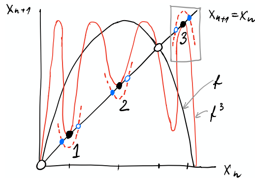
Figure 14: A period-3 orbit can be found in the period-3 window of the orbit diagram. Hollow bullets correspond to unstable period- p points, filled bullets to the stable ones. The dashed and continuous curves shown within the grey rectangle is a smaller distorted copy of map f in its entirety.
