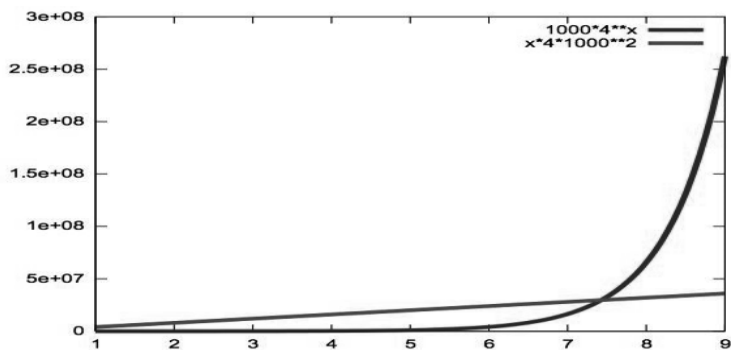
Figure 2: Computation comparison for BruteForce and Pareto for 9 areas.
