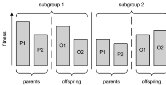
a) After reproduction and mutation a new sets of individuals (offspring) are formed in each subpopulation
