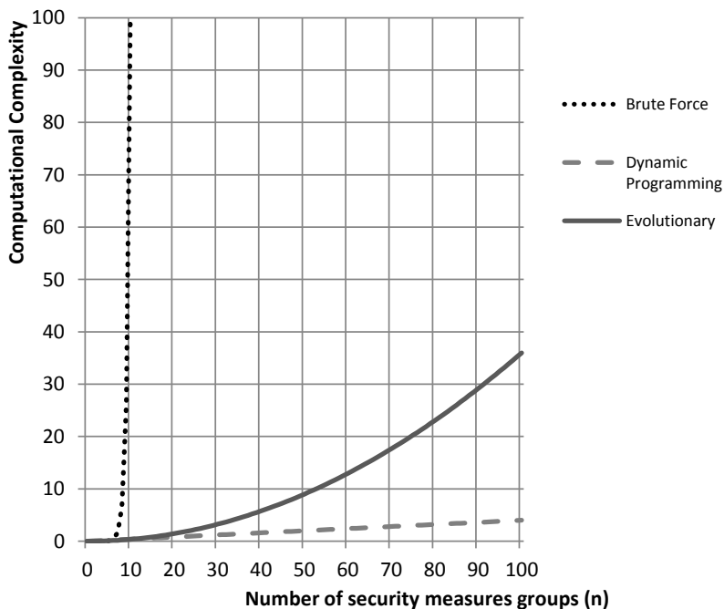
Figure 10. Computational complexities for optimization algorithms used.
