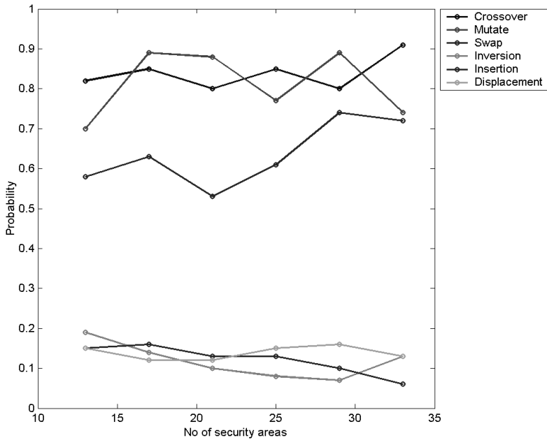
Figure 8: Change of probability of variation operators
