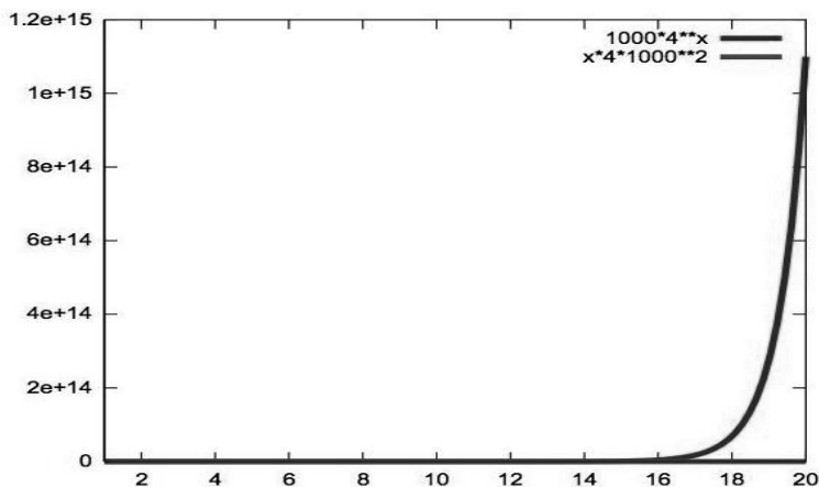
Figure 3: Computations comparison for BruteForce and Pareto for 20 areas.
