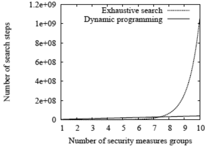
Figure 3. Complexity of search.
