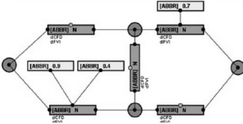
Figure 3: Graph structure used as a test-case in CoCoViLa
