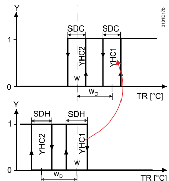
Changeover (P001 = 2 or P001 = 3, P254 = 1) (swap function)
